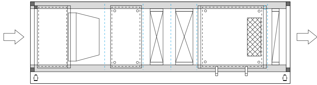
Possible configuration of UTA for wine cellar
